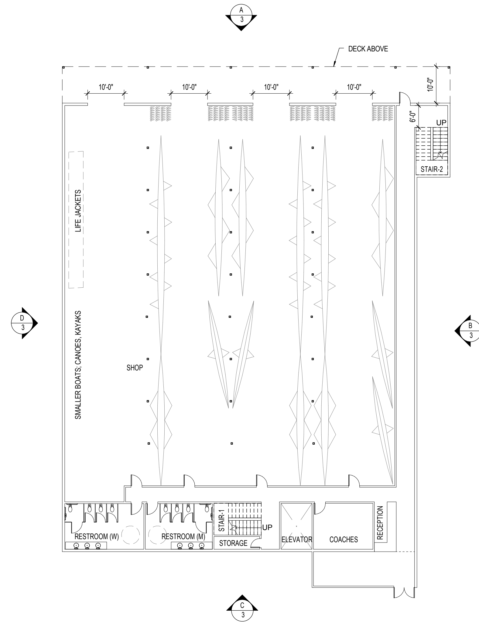
LOWER LEVEL
